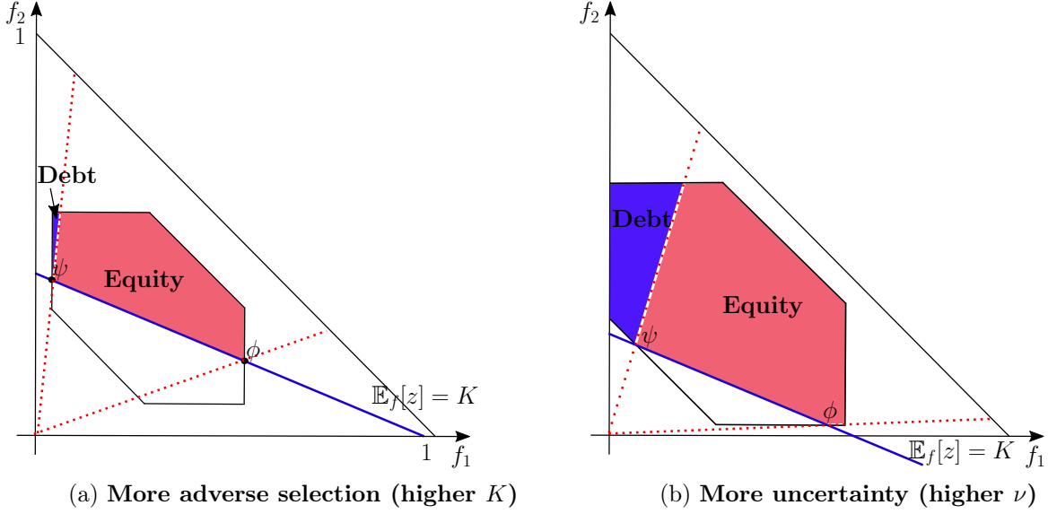
Figure 6: The effect of an increase in the investment level K and the uncertainty \nu In both cases, compared to Figure 5, the share of types who issue equity in equilibrium increases. The set E of types that issue equity is the intersection of B_+ and the cone generated by \psi and \phi , and this cone expands as K or \nu increase, which leads to the dominance of equity for sufficiently large K and \nu .
