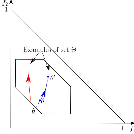
Figure 8: Examples of set \Theta in Nachman and Noe (1994)
